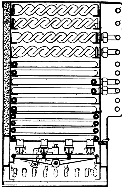
FIG. 345.—Later Form of the Serpollet Flash Generator, consisting of three layers of tubing. The four lowest tiers shown form a coil into which the feed water is injected; the second series of six tiers are arranged "zig-zag," like the nested tubes shown in Fig. 344; the third, or topmost, series of four tiers are also arranged "zig-zag," but are flattened and then twisted as shown.
